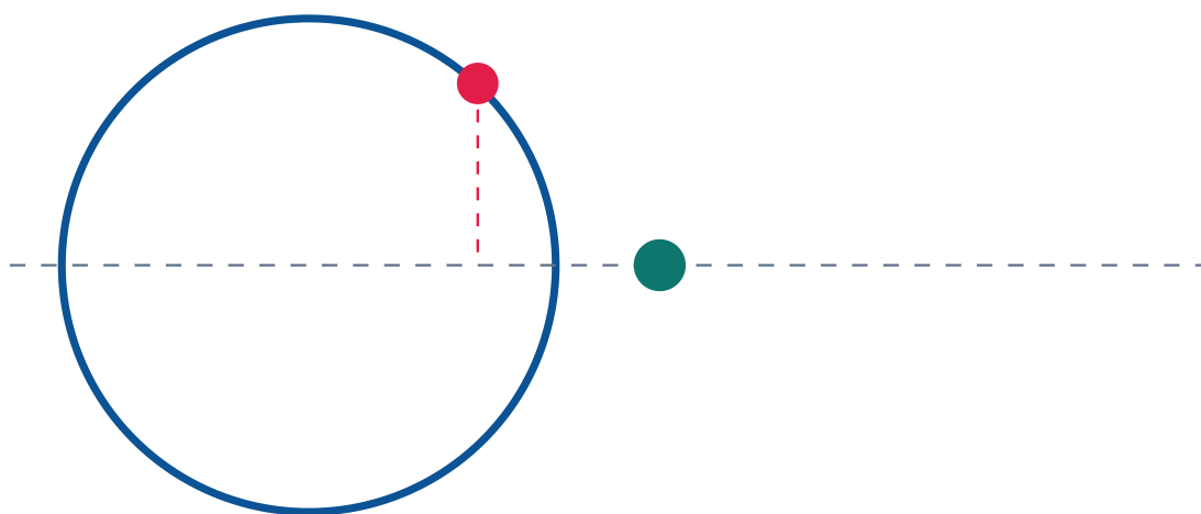
Projection on diameter performs SHM
