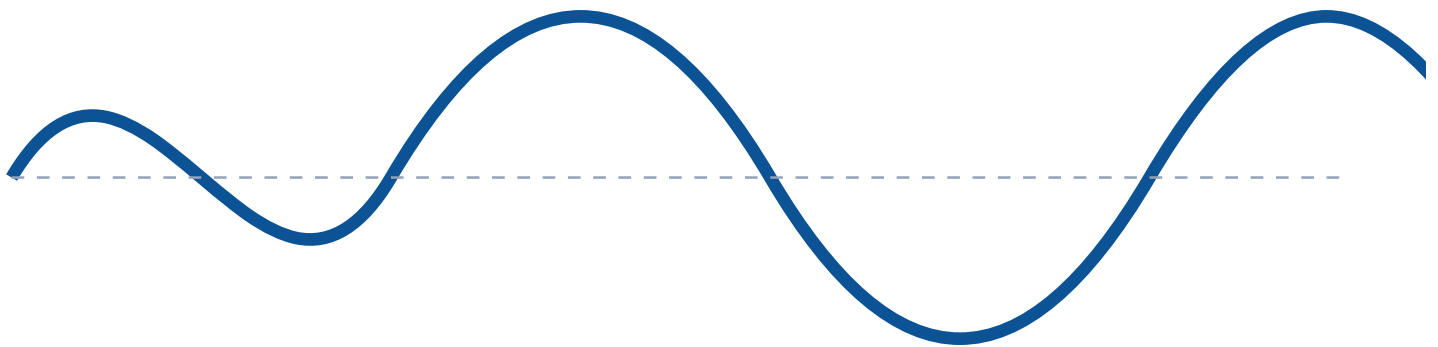
Transverse wave
