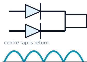
Centre-tapped full-wave
