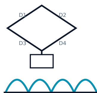
Bridge
