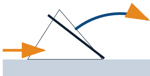
Oblique cutting: chip flows sideways
