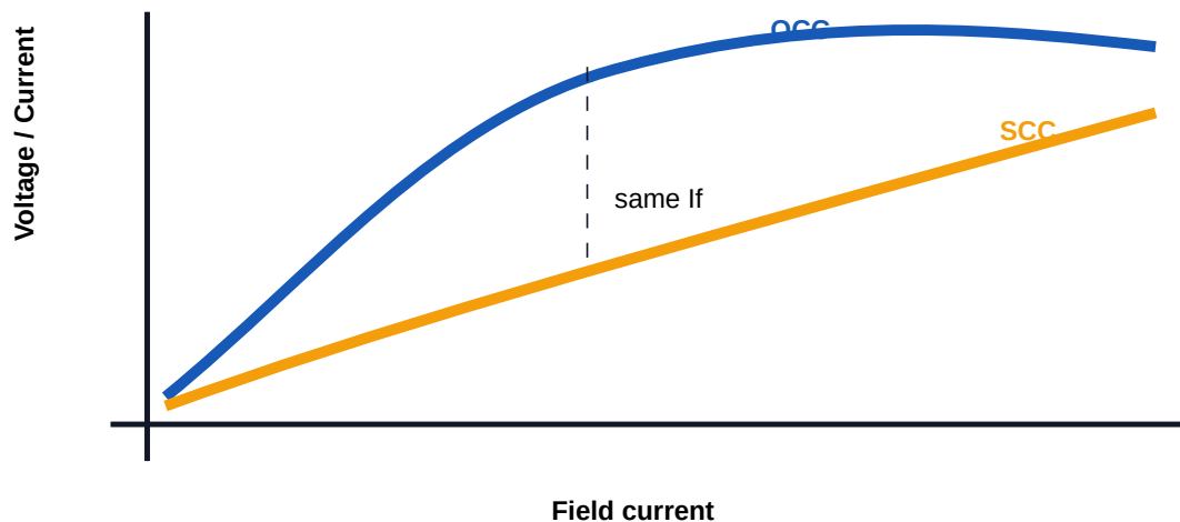
Open circuit and short circuit characteristics
