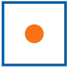
BCC
