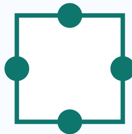
FCC
