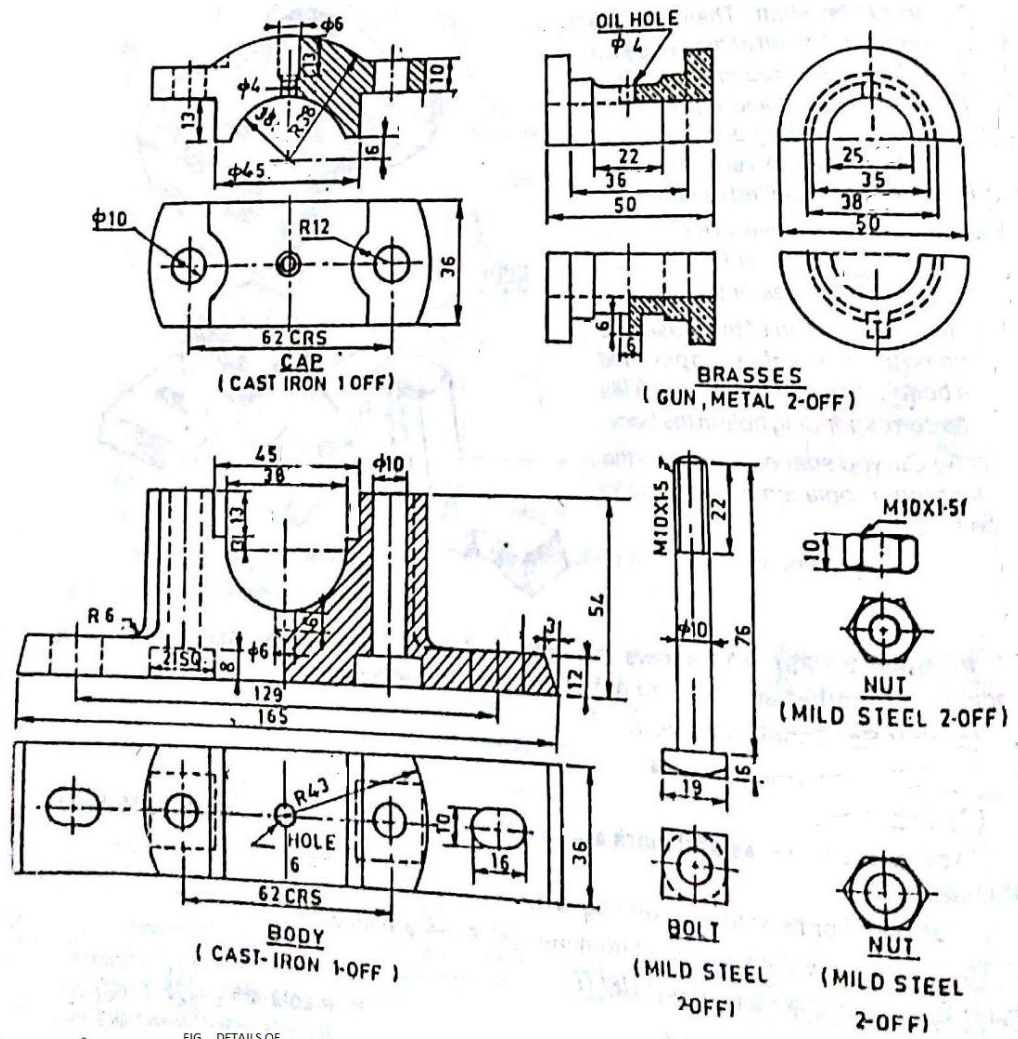
FIG. DETAILS OF PLUMER BLOCK
