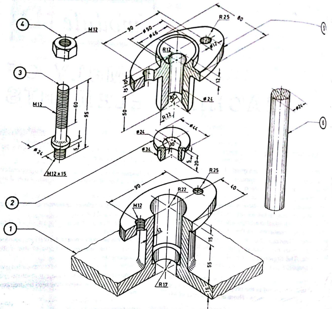
Fig. III Details of stuffing box
