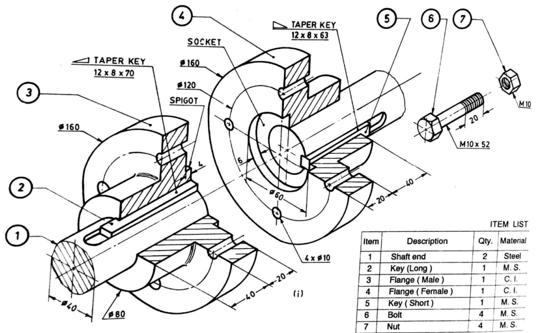
Fig.II Flanged coupling (Un protected type)
