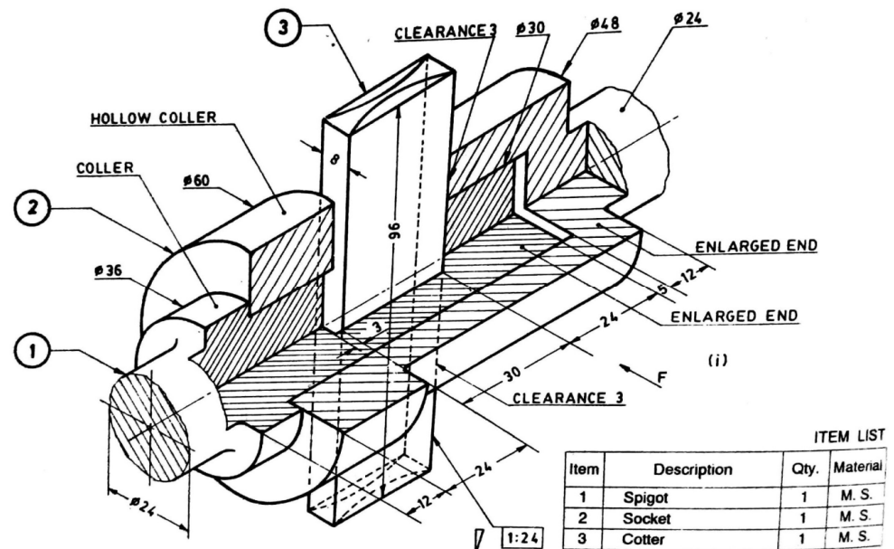
Fig . I Socket and spigot joint
