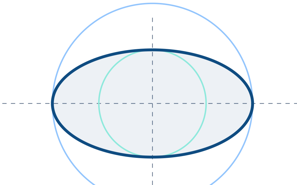
Ellipse by concentric circle idea
