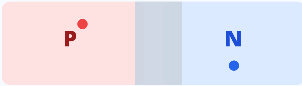
Depletion region
