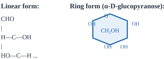
Fig. 2.1 — Glucose: linear (left) and ring (pyranose) forms.
