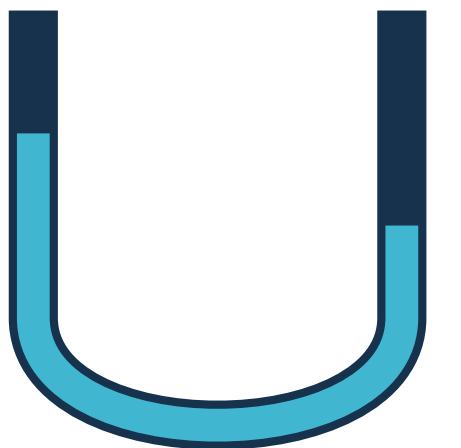
U-tube: \Delta p = \rho g \Delta h
