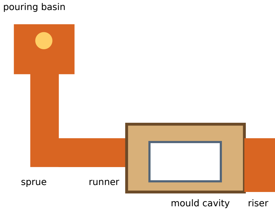
Figure 24. Sand casting system. Reproduce the essential parts, labels and arrows in examination drawings.
