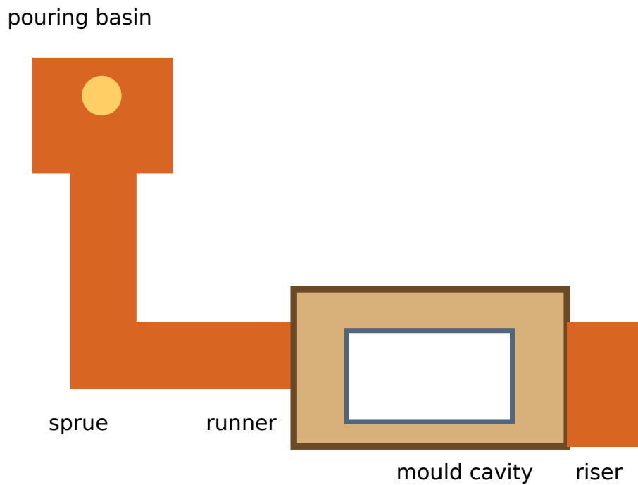
Figure 25. Moulding tools and components. Reproduce the essential parts, labels and arrows in examination drawings.
