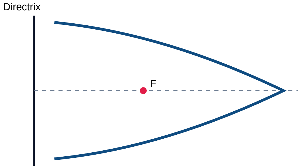
Parabola focus-directrix relation
