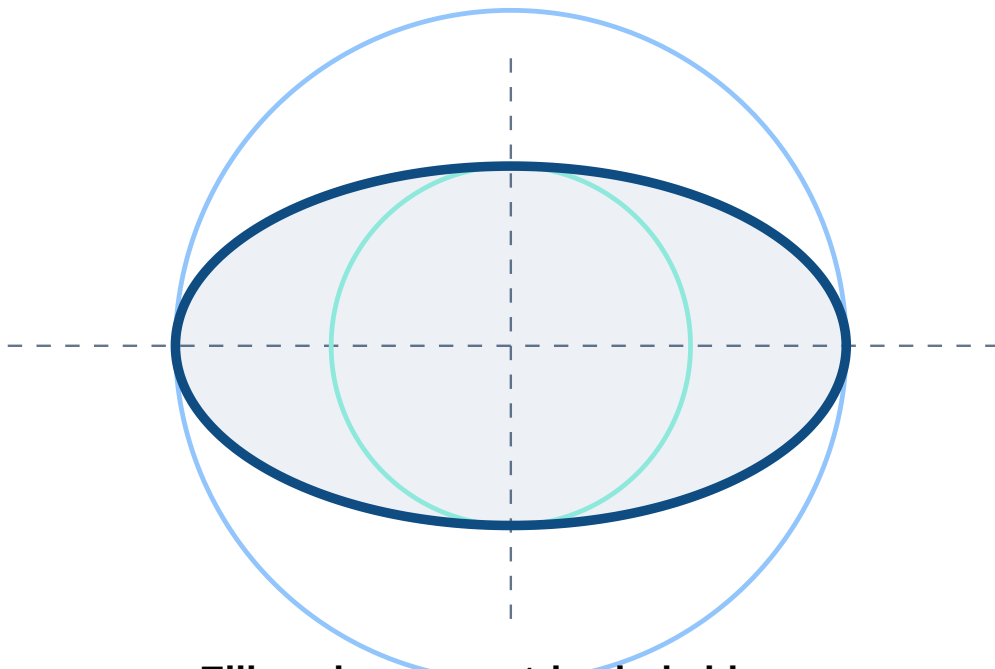
Ellipse by concentric circle idea
