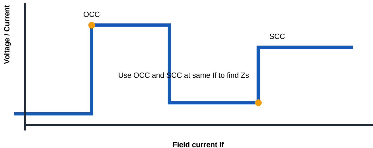
OCC/SCC idea for synchronous impedance
