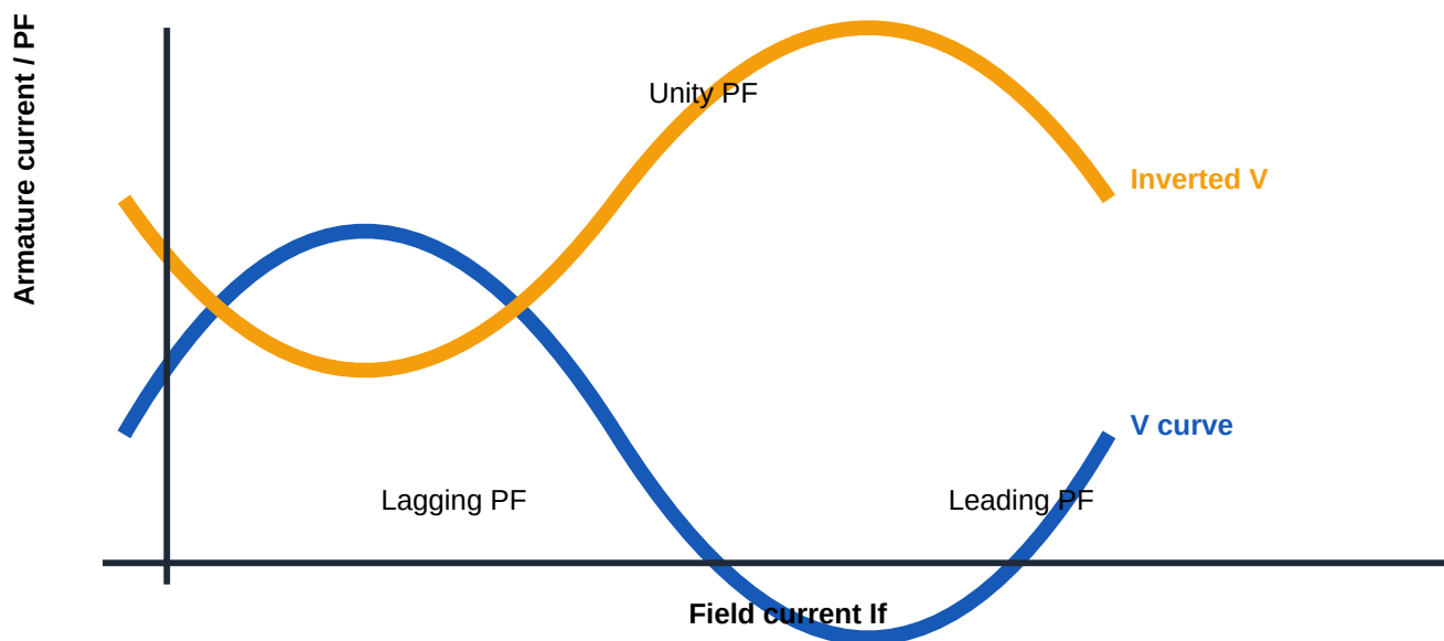
Synchronous motor V and inverted V curves
