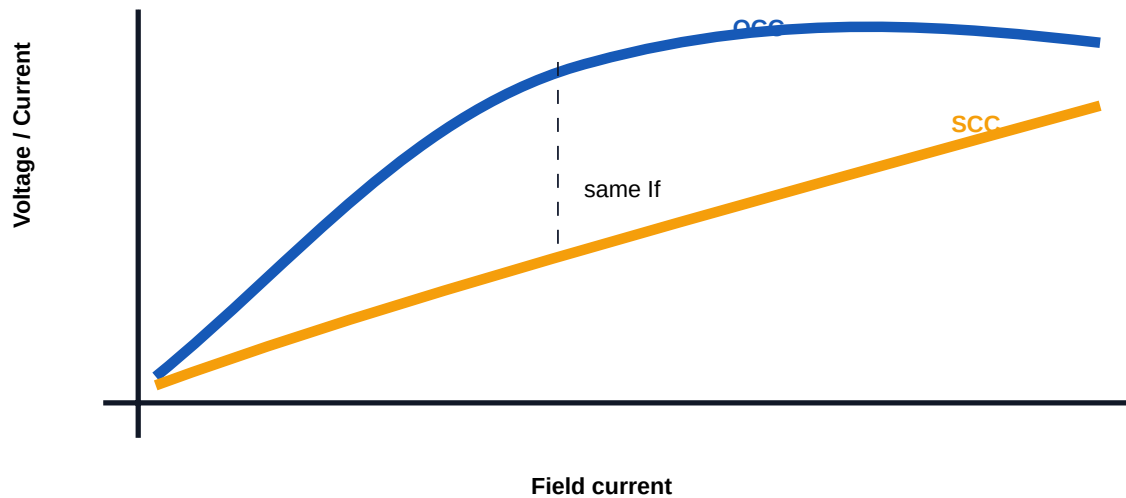
Open circuit and short circuit characteristics
