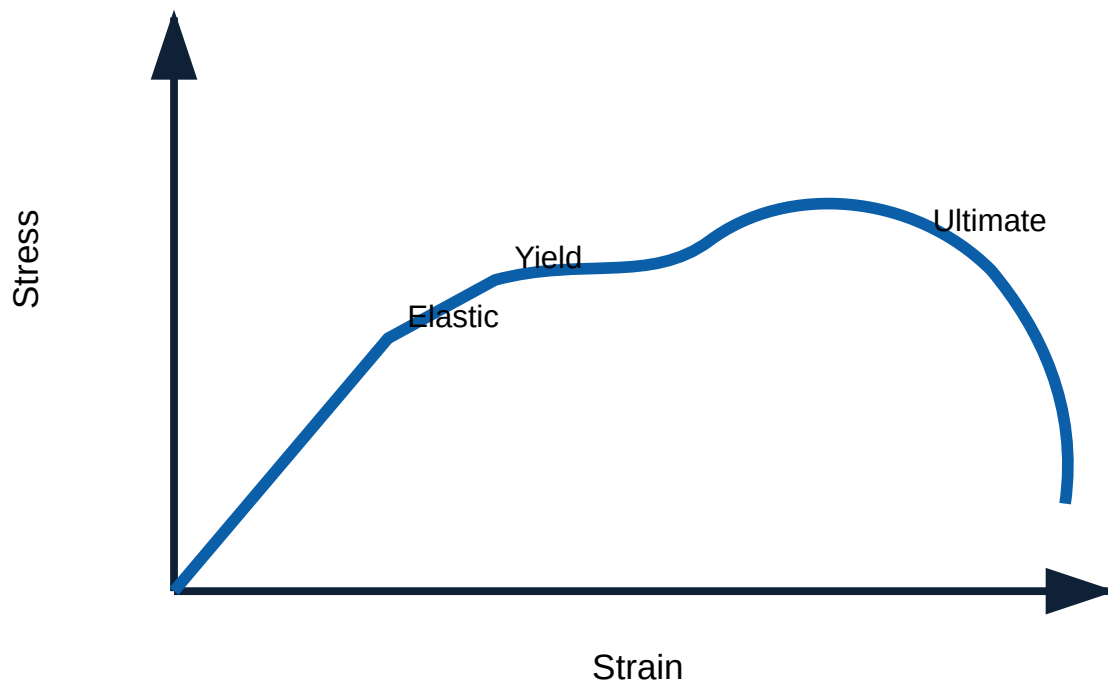
Mild steel stress-strain curve.
