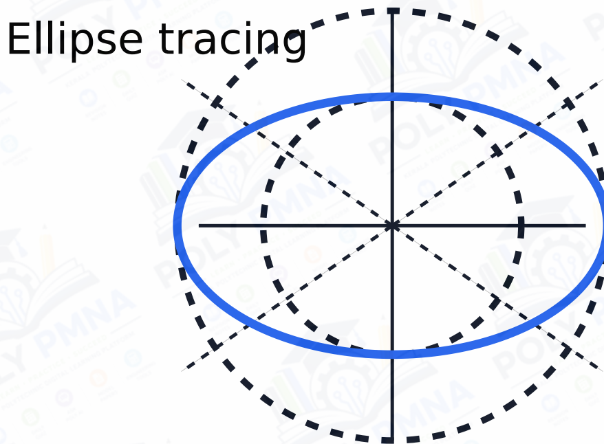
Fig: Ellipse construction using concentric circles.
