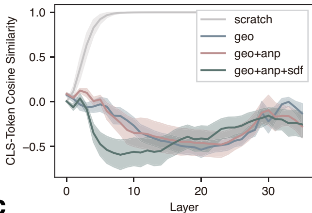
CLS-Token Cosine Similarity vs. Layer
