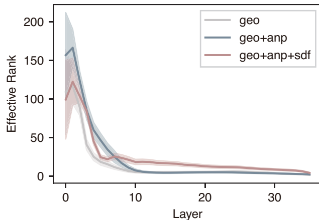
Effective Rank vs. Layer
