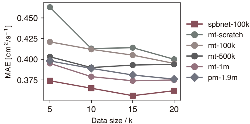
H 2 Diffusivity
