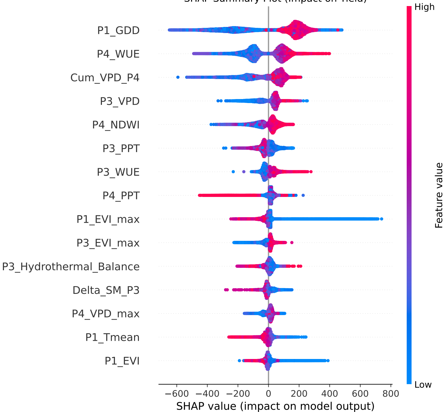
SHAP Summary Plot (Impact on Yield)
