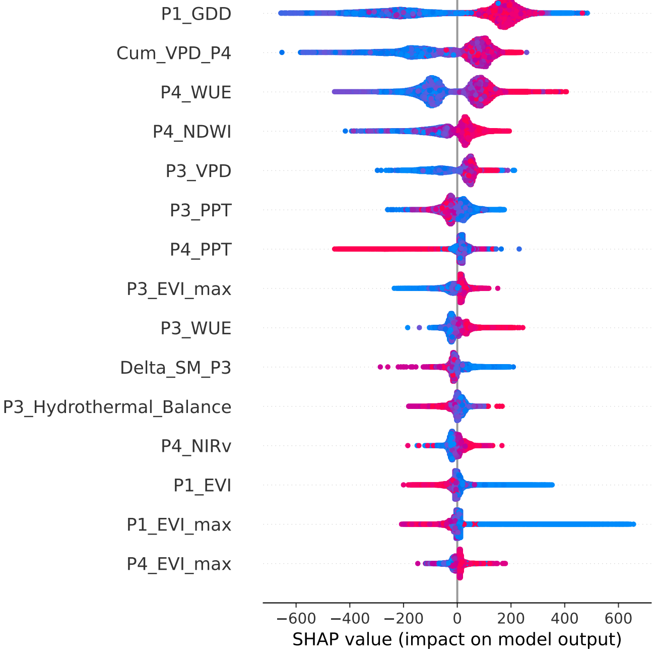
SHAP Summary Plot
