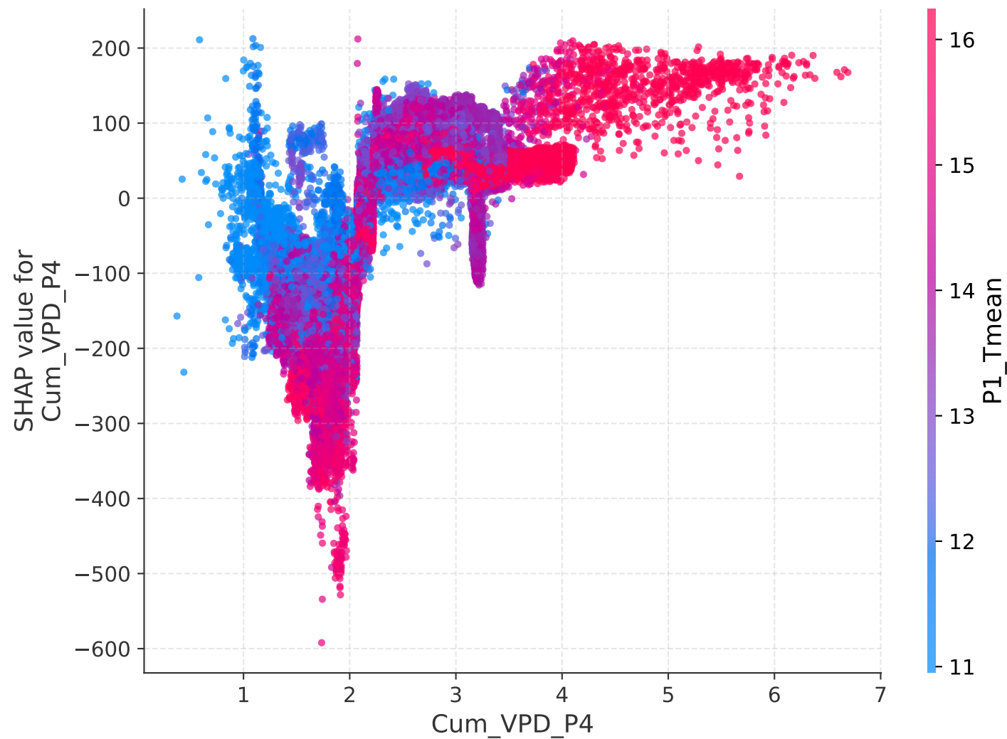
SHAP Dependence Plot: Cum_VPD_P4
