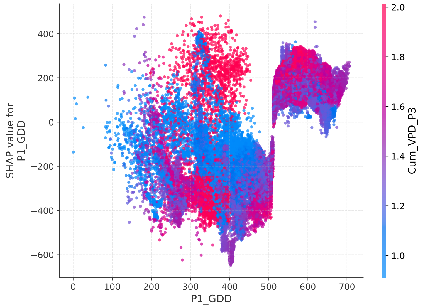
SHAP Dependence Plot: P1_GDD
