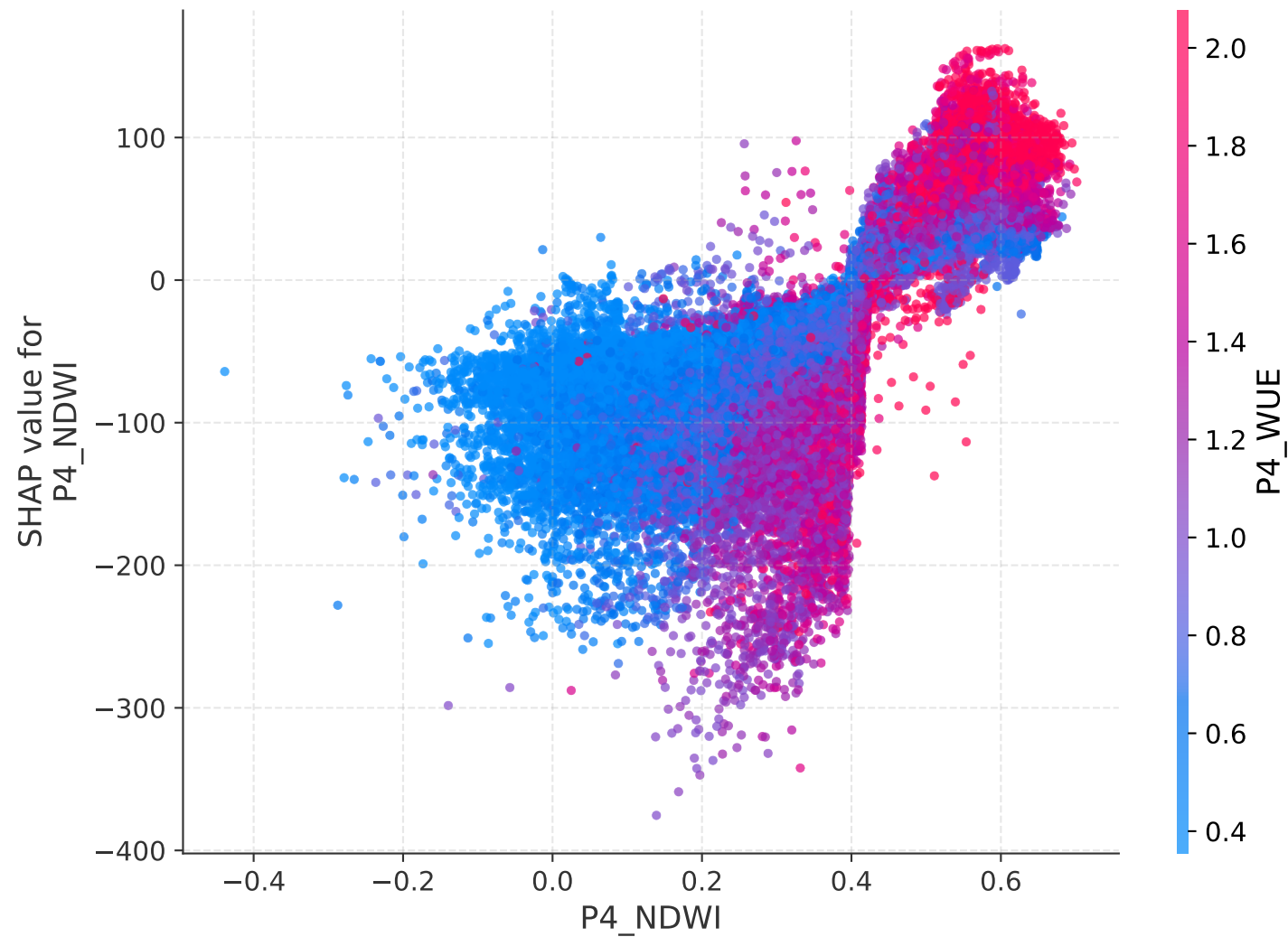
SHAP Dependence Plot: P4_NDWI
