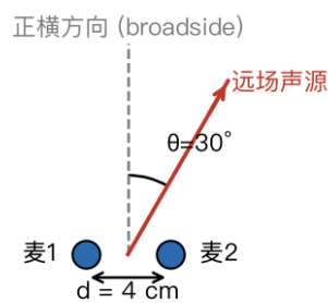
(c) \theta = \arcsin(c \cdot \tau / d) = \arcsin(0.5) = 30^\circ ( \theta 自正横方向起算)
