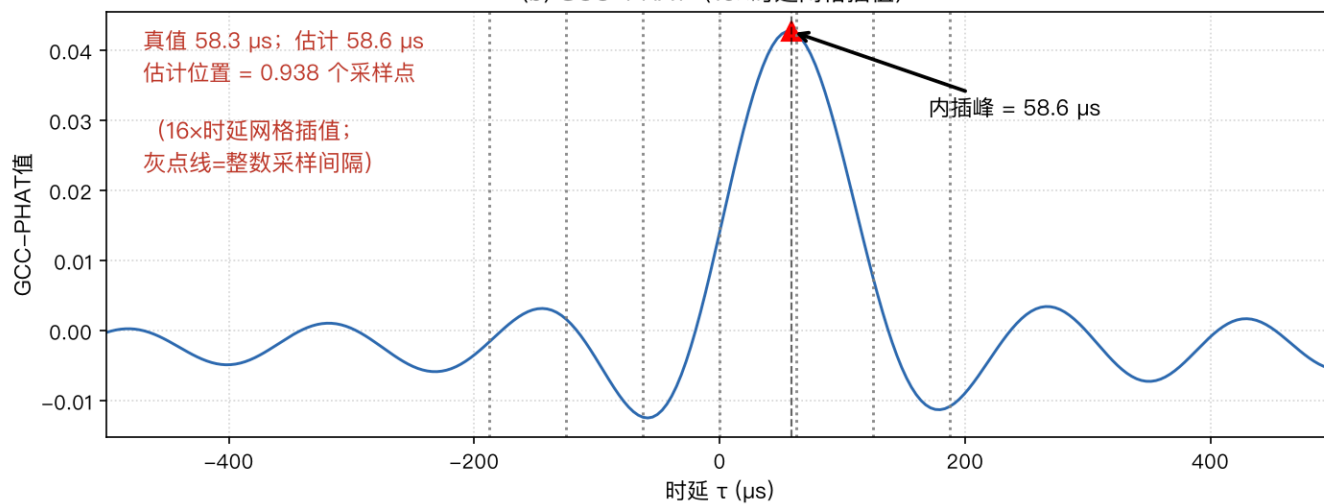
(c) \theta = \arcsin(c \cdot \tau / d) = \arcsin(0.5) = 30^\circ ( \theta 自正横方向起算)
