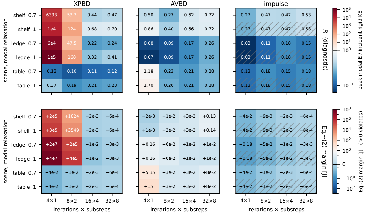
Figure 3: The same contact row in three fixed-budget solver formulations over an identical 24-cell sweep (3 scenes × modal relaxation {0.7, 1.0} × budget), governor OFF. Top: the ratio R = peak modal energy / peak incident rigid kinetic energy, log scale diverging at 1 – a severity diagnostic. XPBD exceeds 1 in 8/24 cells, AVBD in 2/24, the implicit realization in 0/24. Bottom: the invariant itself – the signed margin of (2) in joules, symmetric-log, diverging at 0; positive violates. The two rows disagree on AVBD. Hatched rows mark the relaxation axis, which that formulation does not consume; those rows are bit-identical by construction and shown for grid symmetry, not as independent measurements. We report joules rather than a second ratio because every candidate denominator misleads: supply-so-far explodes in the opening substeps, the run total hides early peaks.
