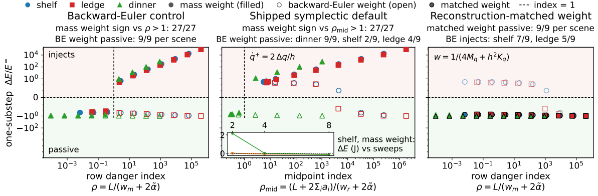
Figure 3: Shipped position-based contact row. Left, backward-Euler control. Middle, host default, where the reconstruction shifts the governing index to \rho_{mid} and the backward-Euler-shaped weight injects. Right, the matched weight 4M_q + h^2 K_q ; inset, injection decays as the budget grows. Hard contact, one sweep, cold start, e = 0 .
