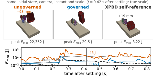
Figure 1: One shelf impact at a production-like interactive budget (1 \times 8), true scale, three independent runs. Ungoverned, truncation energy throws the resting books up to 93 mm — more than their own height; governed, (2) holds peak modal energy to 29.5 J and they stay within 1 mm of rest; the reference is the host's own high-iteration self-reference (500 \times ). The bound removes the spurious launch and some legitimate motion with it: the reference lifts one book 19 mm, the governed run none.
