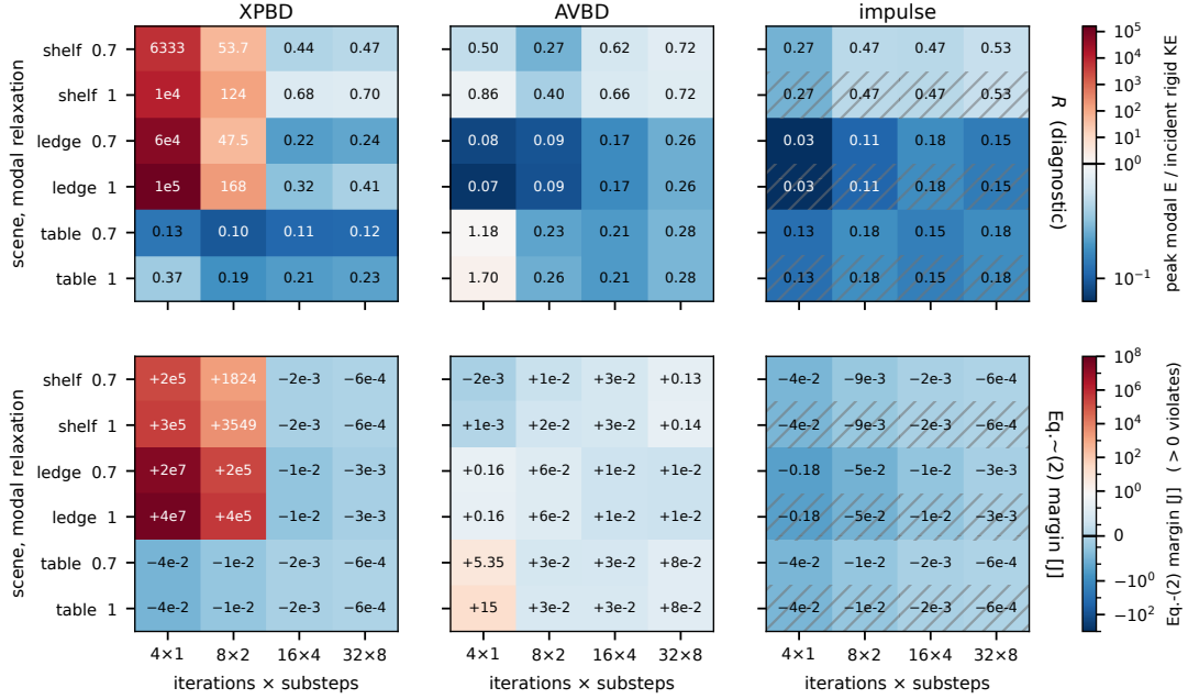
Figure 2: The same contact row in three fixed-budget solver implementations over an identical 24-cell sweep (3 scenes × modal relaxation {0.7, 1.0} × budget), governor OFF. Top: the ratio R = \text{peak modal energy} / \text{peak incident rigid kinetic energy} , log scale diverging at 1 — a severity diagnostic. XPBD exceeds 1 in 8/24 cells, AVBD in 2/24, the implicit realization in 0/24. Bottom: the invariant itself — the signed margin of (2) in joules, symmetric-log, diverging at 0; positive values violate. The two panels disagree on AVBD. Hatched rows mark a relaxation axis the host does not consume, bit-identical by construction (§3.1).
