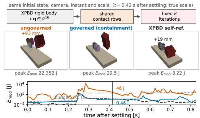
Figure 1: One shelf impact at a production-like interactive budget (1×8), true scale, three independent runs. Ungoverned, truncation energy throws the resting books up to 93 mm, more than their own height. Governed, (2) holds peak modal energy to 29.5 J and the books stay within 1 mm of rest; the reference is the host's own high-iteration run (500×1). The bound removes the spurious launch and some legitimate motion with it: the reference lifts one book 19 mm, the governed run none.
