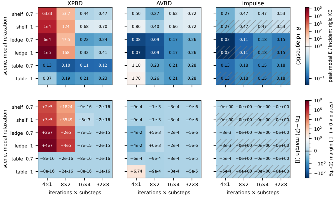
Figure 2: The same contact row in three fixed-budget solver implementations over an identical 24-cell sweep (3 scenes \times modal relaxation {0.7, 1.0} \times budget), governor OFF. Top: the ratio R = peak modal energy / peak incident rigid kinetic energy, log scale diverging at 1 — a severity diagnostic. XPBD exceeds 1 in 8/24 cells, AVBD in 2/24, the implicit realization in 0/24. Bottom: the invariant itself — the signed margin of (2) in joules, symmetric-log, diverging at 0; positive values violate. The two panels disagree on AVBD. Hatched rows mark a relaxation axis the host does not consume, bit-identical by construction (§3.1).
