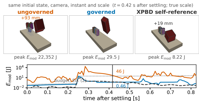
Figure 1: One shelf impact at a production-like interactive budget ( 1 \times 8 ), true scale, three independent runs. Ungoverned, truncation energy throws the resting books up to 93 mm — more than their own height; governed, (2) holds peak modal energy to 29.5 J and they stay within 1 mm of rest; the reference is the host's own high-iteration self-reference ( 500 \times 1 ). The bound removes the spurious launch and some legitimate motion with it: the reference lifts one book 19 mm, the governed run none.
