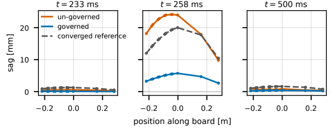
Figure 1: The deflected support surface through one impact at a starved budget ( 8 \times 2 ), sampled at the 48 support contact rows: d_i = U_y[i]^T \mathbf{q} , the quantity (1) sees. Un-governed, the board reaches 24.1 mm of sag against the converged reference's 20.0; governed, the bound holds peak modal energy to 29.3 J but takes the legitimate sag down with the spurious ring, to 5.9 mm. A non-diverging result, not a faithful one (§3.3).
