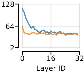
Math
