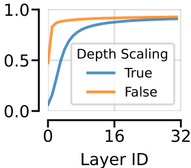
Math
