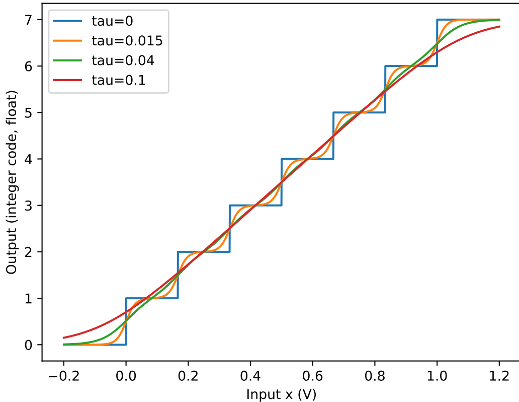
Soft integer-code output vs input for different temperatures
