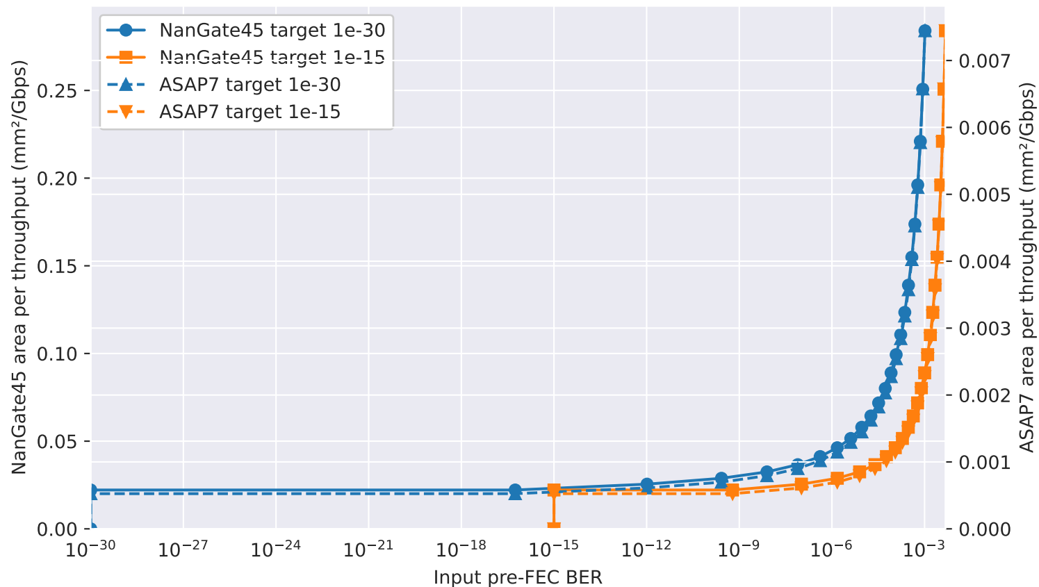
FEC Area per Throughput vs Raw BER (Targets 1e-30, 1e-15)
