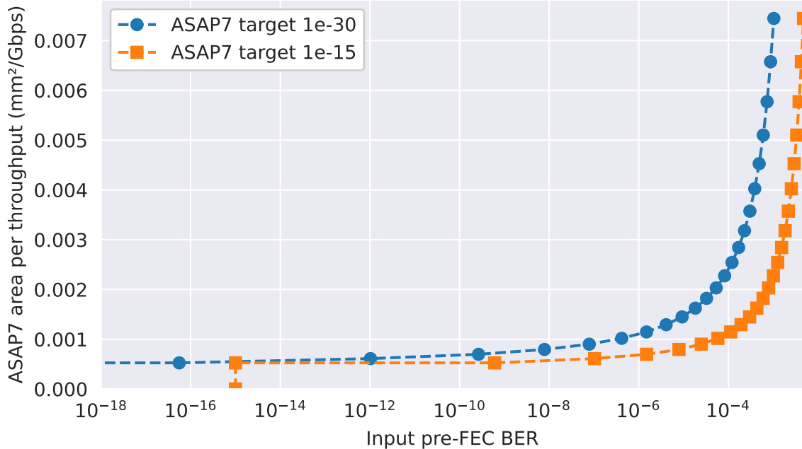
FEC Area per Throughput vs Raw BER (Targets 1e-30 , 1e-15 )
