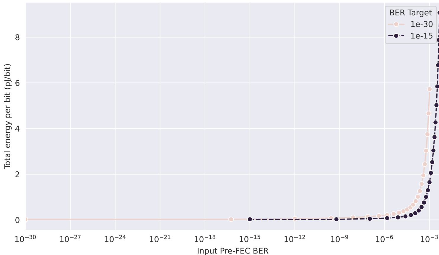
ASAP7 RS(m=8, best-k) Energy/bit vs Input BER (targets: 1e-30, 1e-15)
