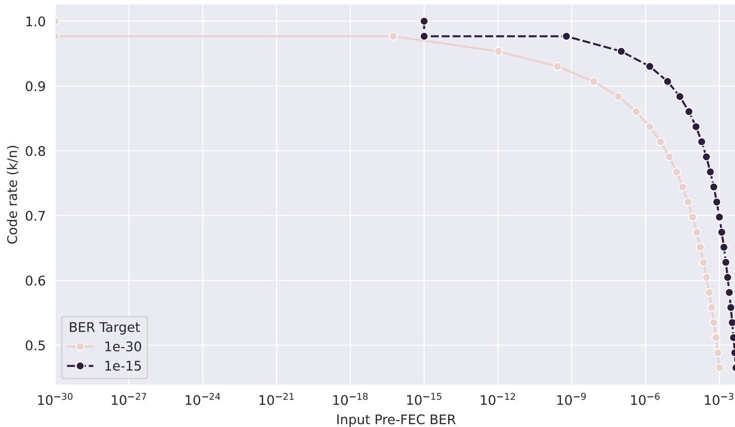
ASAP7 RS(m=8, best-k) Rate vs Input BER (targets: 1e-30, 1e-15)
