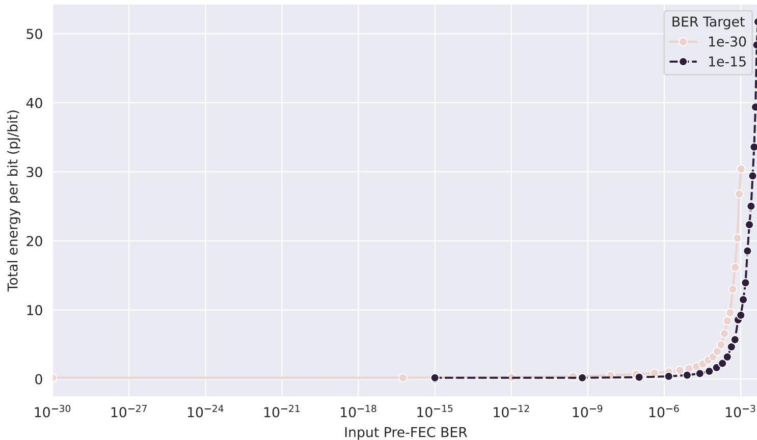
NanGate45 RS(m=8, best-k) Energy/bit vs Input BER (targets: 1e-30, 1e-15)
