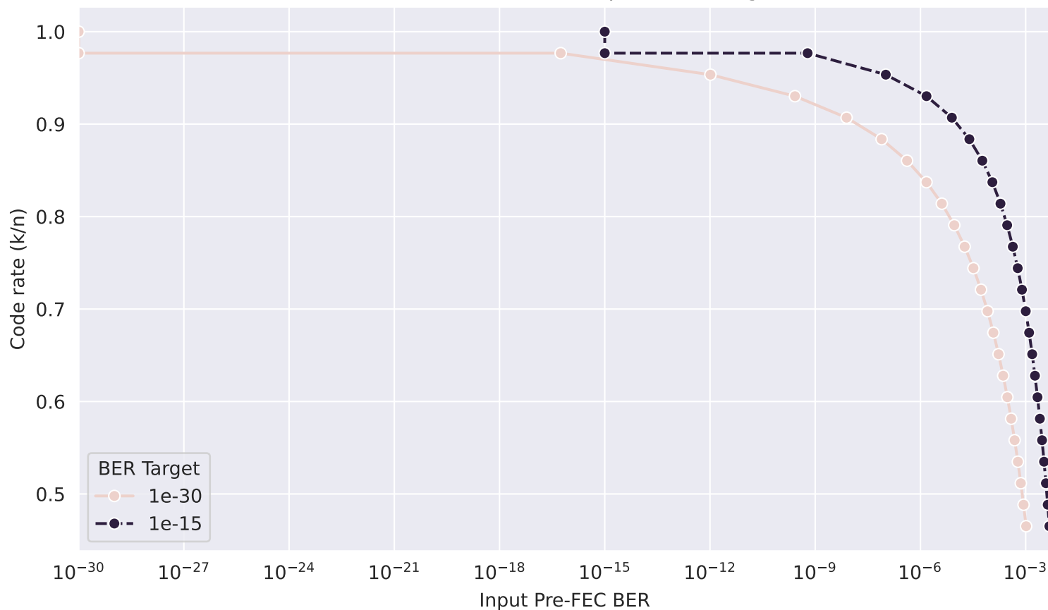
NanGate45 RS(m=8, best-k) Rate vs Input BER (targets: 1e-30, 1e-15)
