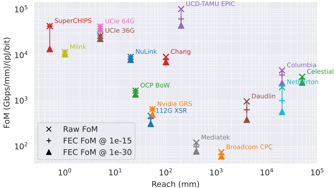
Reach vs FoM (Raw vs FEC @ 1e-15, 1e-30)
