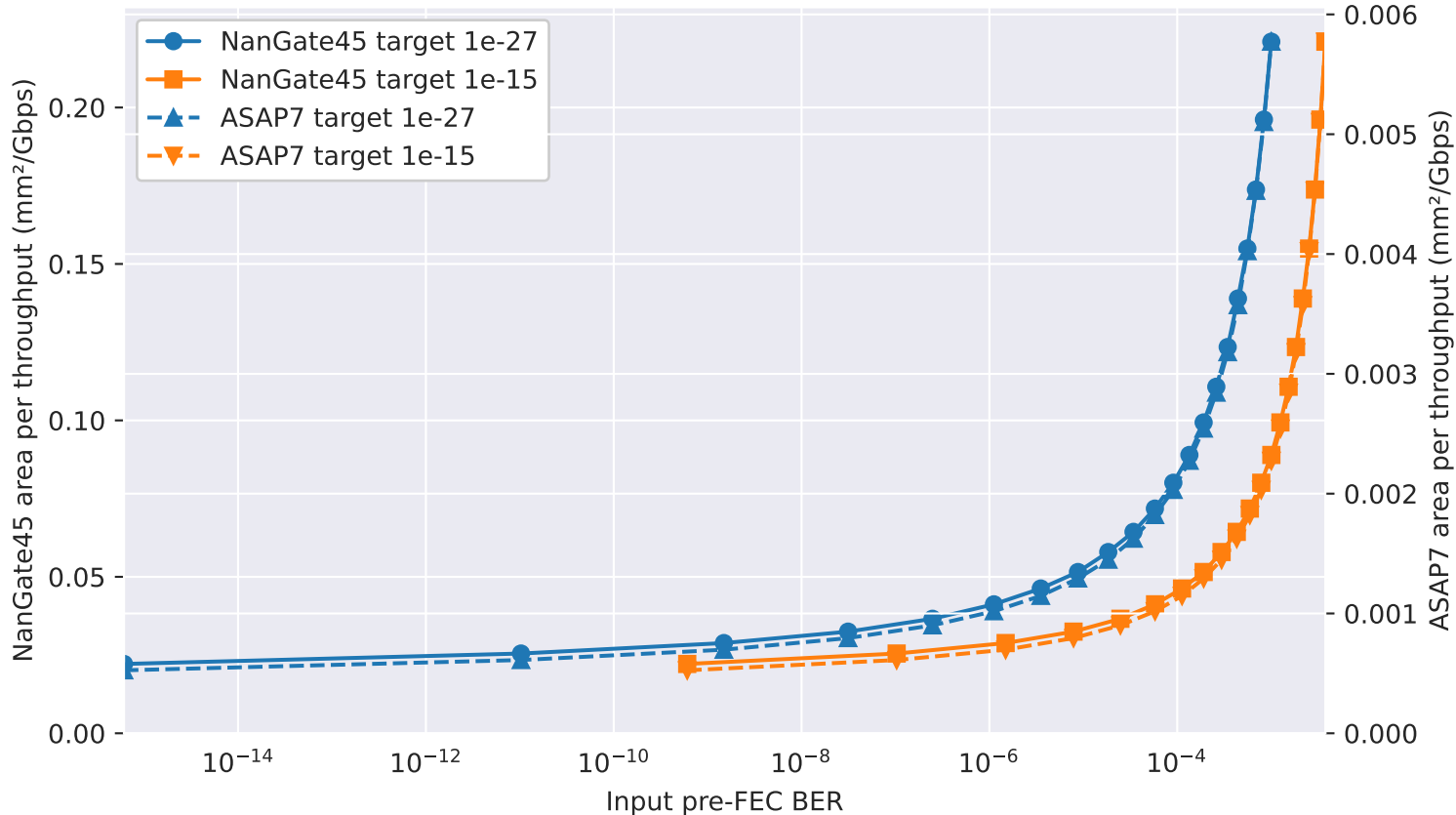
FEC Area per Throughput vs Raw BER (Targets 1e-27, 1e-15)
