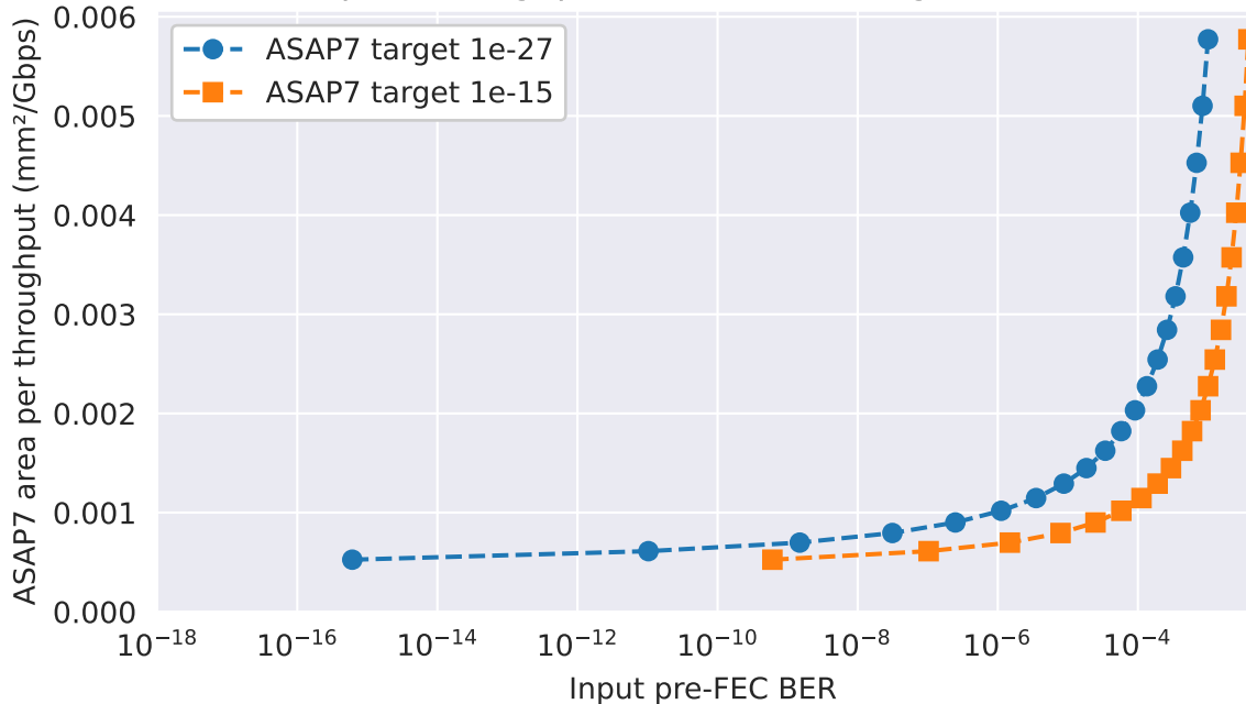
FEC Area per Throughput vs Raw BER (Targets 1e-27 , 1e-15 )
