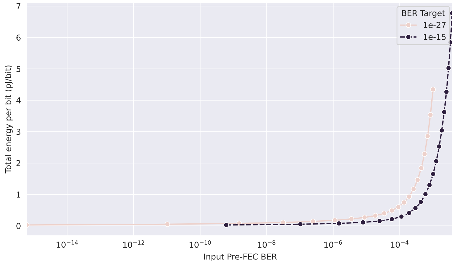
ASAP7 RS(m=8, best-k) Energy/bit vs Input BER (targets: 1e-27, 1e-15)
