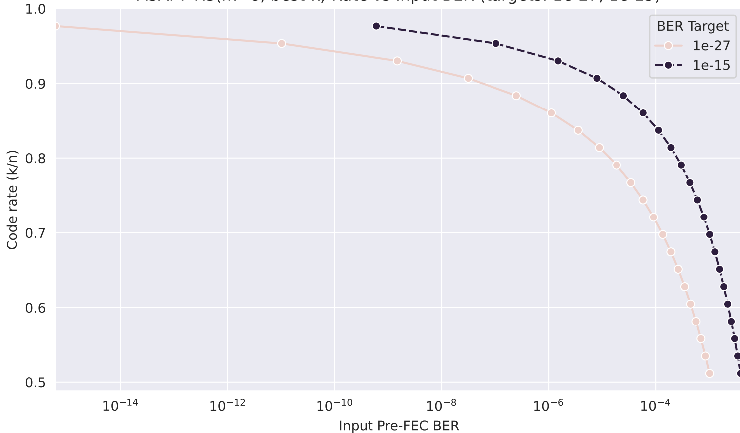
ASAP7 RS(m=8, best-k) Rate vs Input BER (targets: 1e-27, 1e-15)
