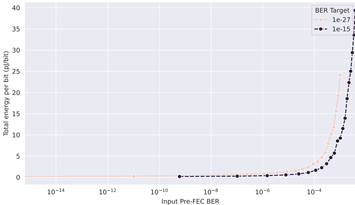
NanGate45 RS(m=8, best-k) Energy/bit vs Input BER (targets: 1e-27, 1e-15)
