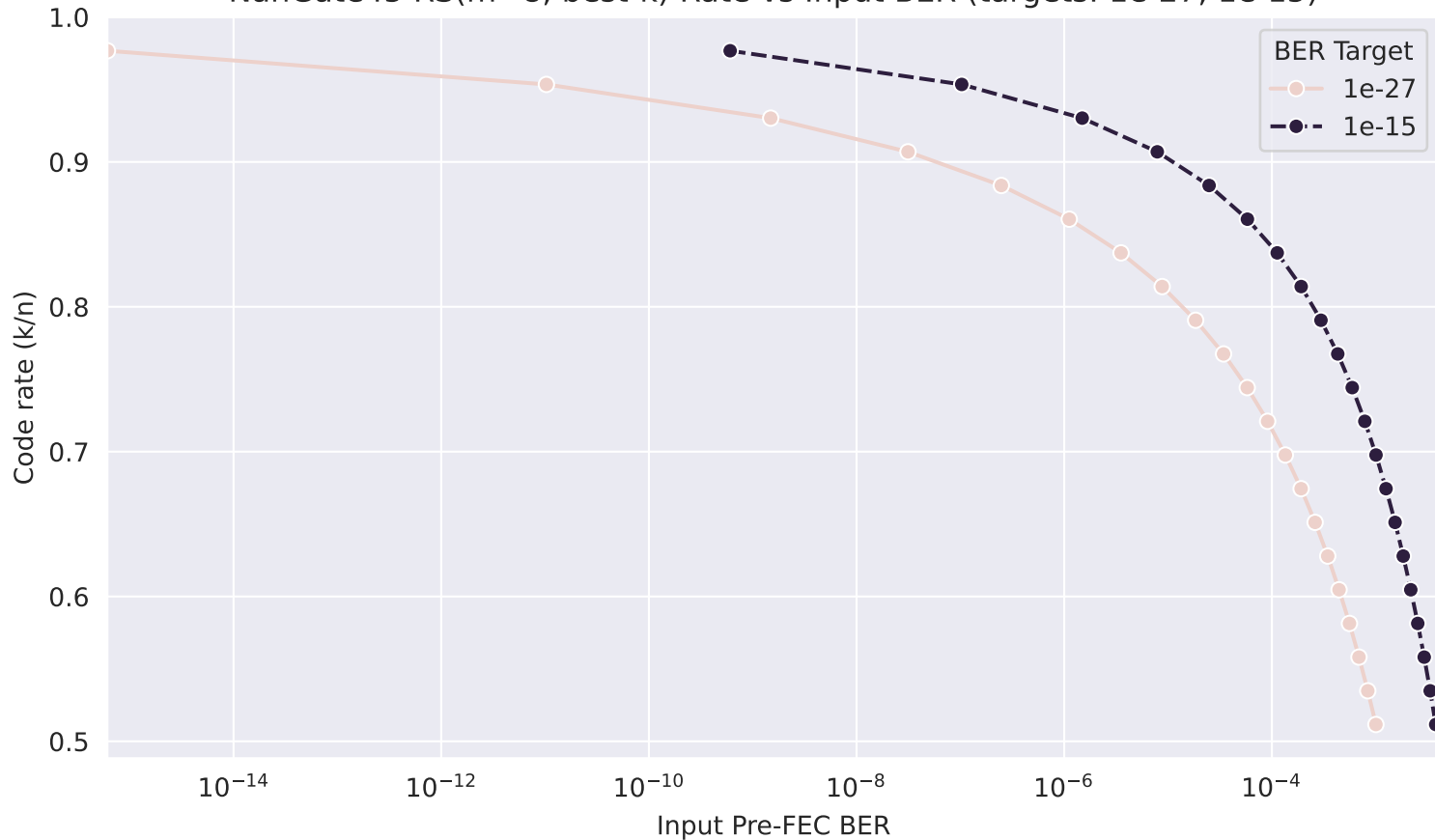
NanGate45 RS(m=8, best-k) Rate vs Input BER (targets: 1e-27, 1e-15)
