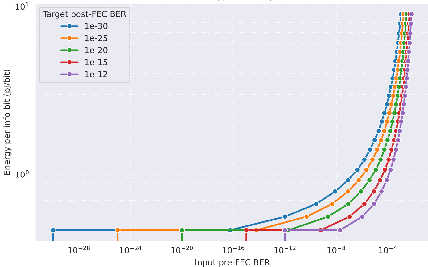
RS Decoder p j /bit vs Input BER
