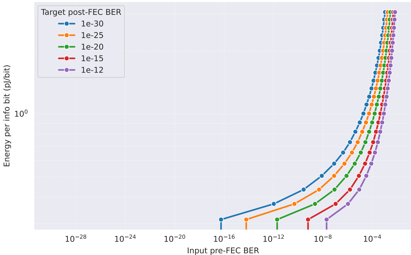
RS Decoder pJ/bit vs Input BER
