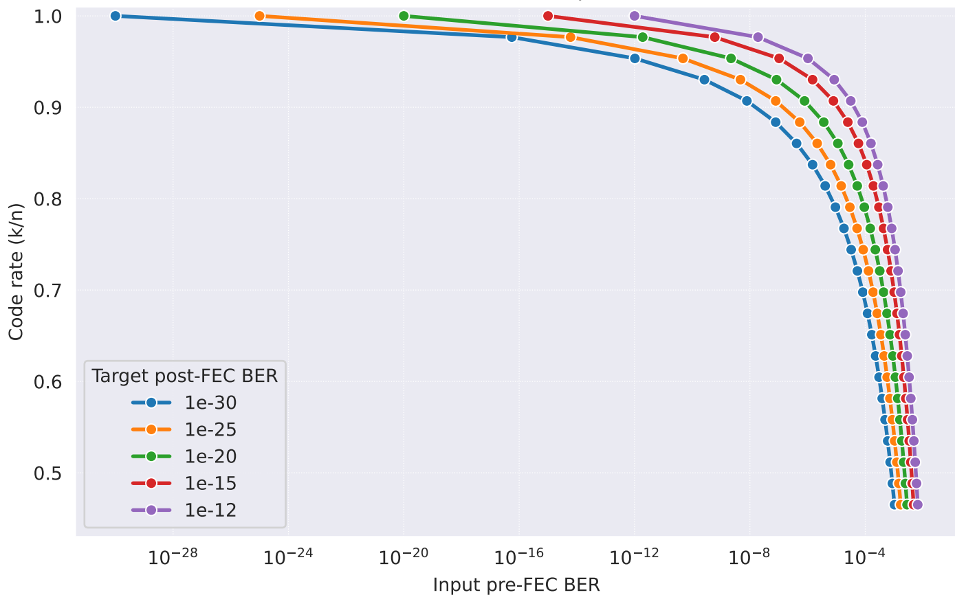
RS Code Rate vs Input BER
