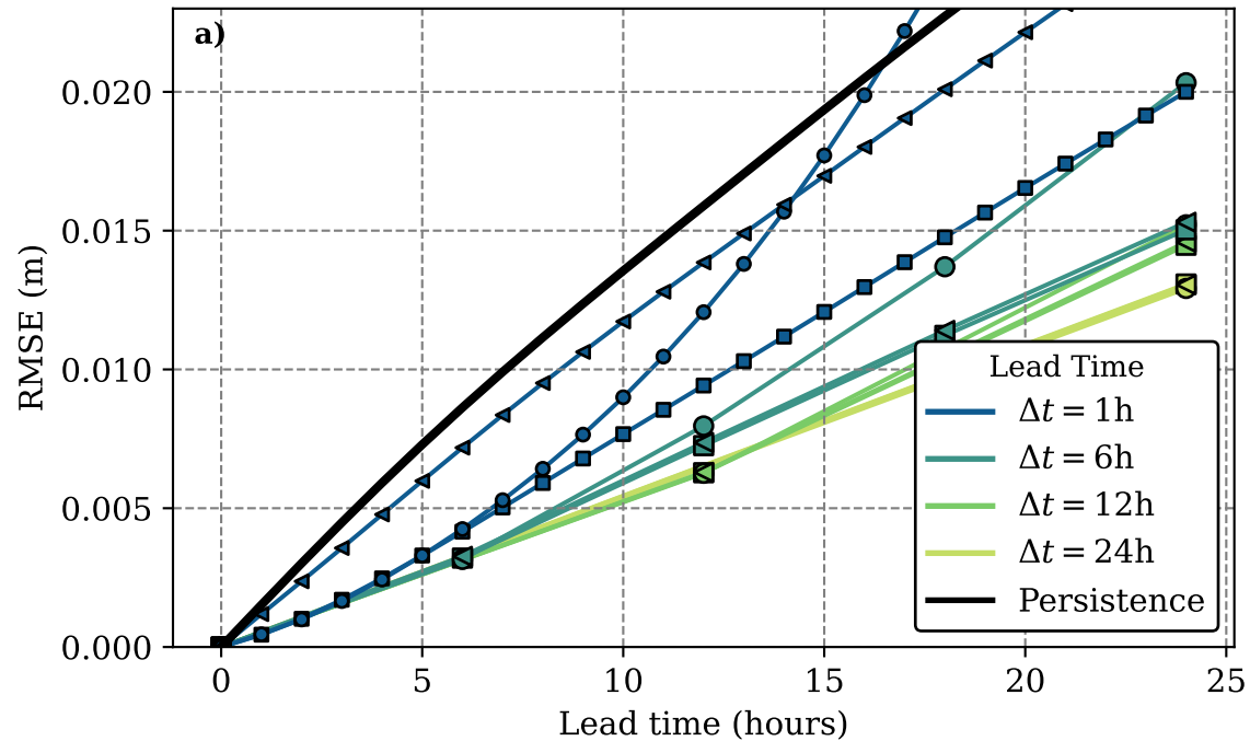
SIV 1 day forecast on full Arctic
